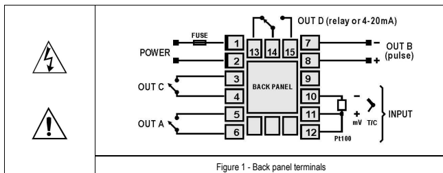
Figure 1 - Back panel terminals
