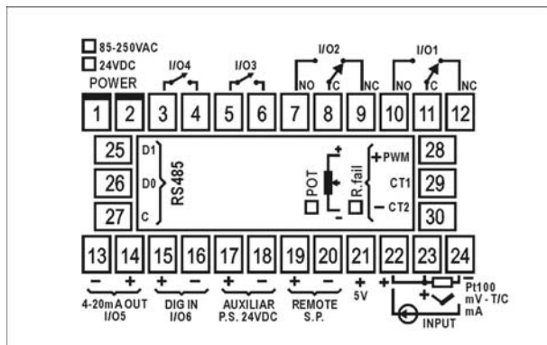
Figure 2 - Backpanel terminals
